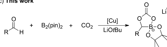
Figure 1. a) Synthesis of cyclic carbonates by coupling of epoxide and CO 2 . b) Synthesis of lithium bis(oxalato)borate (LiBOB) from complicated starting materials. c) One-pot synthesis of lithium borate-carbonate ion pairs containing a unique boron-implanted cyclic carbonate structure from easily available starting materials.
